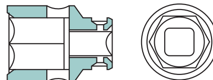
43mm HEXAGON
