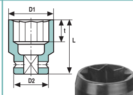
8 POINT IMPACT SOCKETS REGULAR LENGTH
