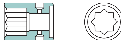
30mm DOUBLE SQUARE
