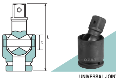
UNIVERSAL JOINT
