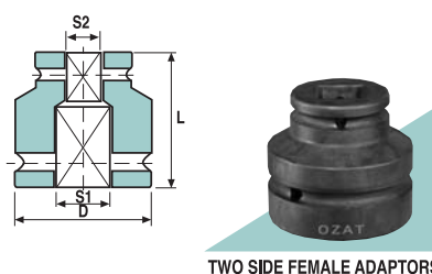
TWO SIDE FEMALE ADAPTORS
