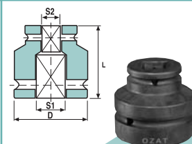
TWO SIDE FEMALE ADAPTORS
