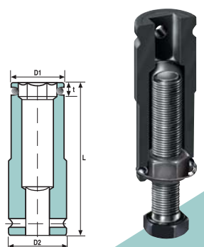
STANDARD / LONG
