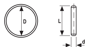
RETAINING PINS AND RING
