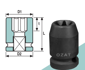
SURFACE DRIVE IMPACT SOCKETS REGULAR LENGTH
