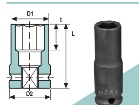
6 POINT THIN WALL IMPACT SOCKETS LONG
