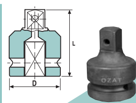
ADAPTORS
