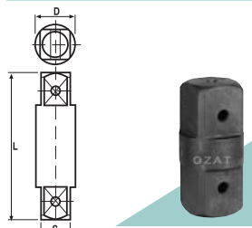
TWO SIDE MALE ADAPTORS
