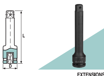
EXTENSIONS
