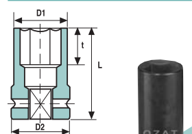
6 POINT THIN WALL IMPACT SOCKETS REGULAR LENGTH
